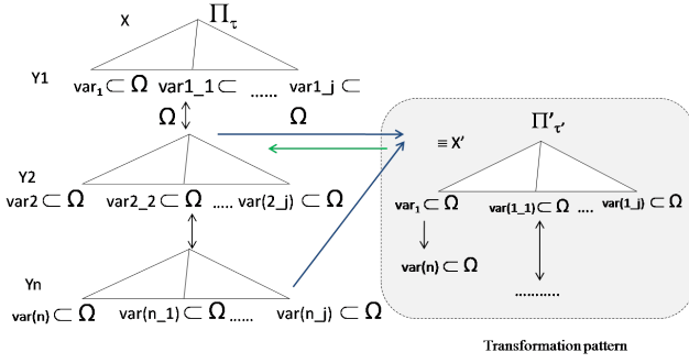
Figure 2: Graphical representation of NKRLs Inferences procedures
