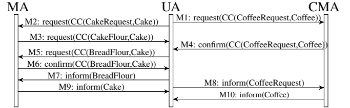
Figure 6: Sequence Diagram for Scenario 2
