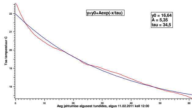
Figure 5. Analysis I (tau is directly related to the room integrated heat capacity).
