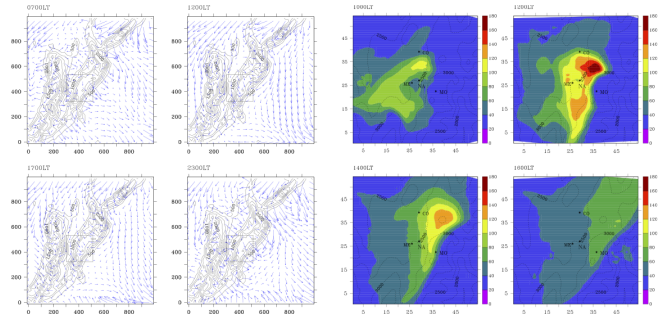
Figure 2: The windfield and the resulting O 3 estimations in the city of Bogota from the physical model TAPOM [29].
