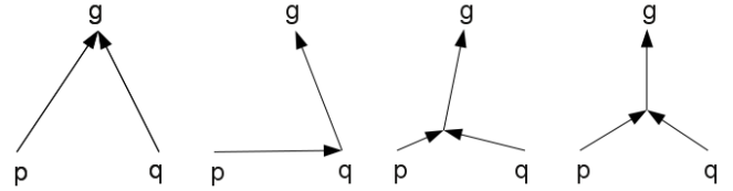
Figure 1: From left to right: Users p and q meet at the destination g , at q 's position, at some intermediate place, at the Torricelli point.
