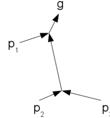
Figure 2: Meeting tree of three individuals p_1, p_2, p_3 heading to a common goal g meeting at intermediate points.
