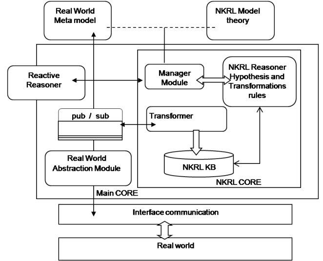
Figure 3: Semantic architecture
